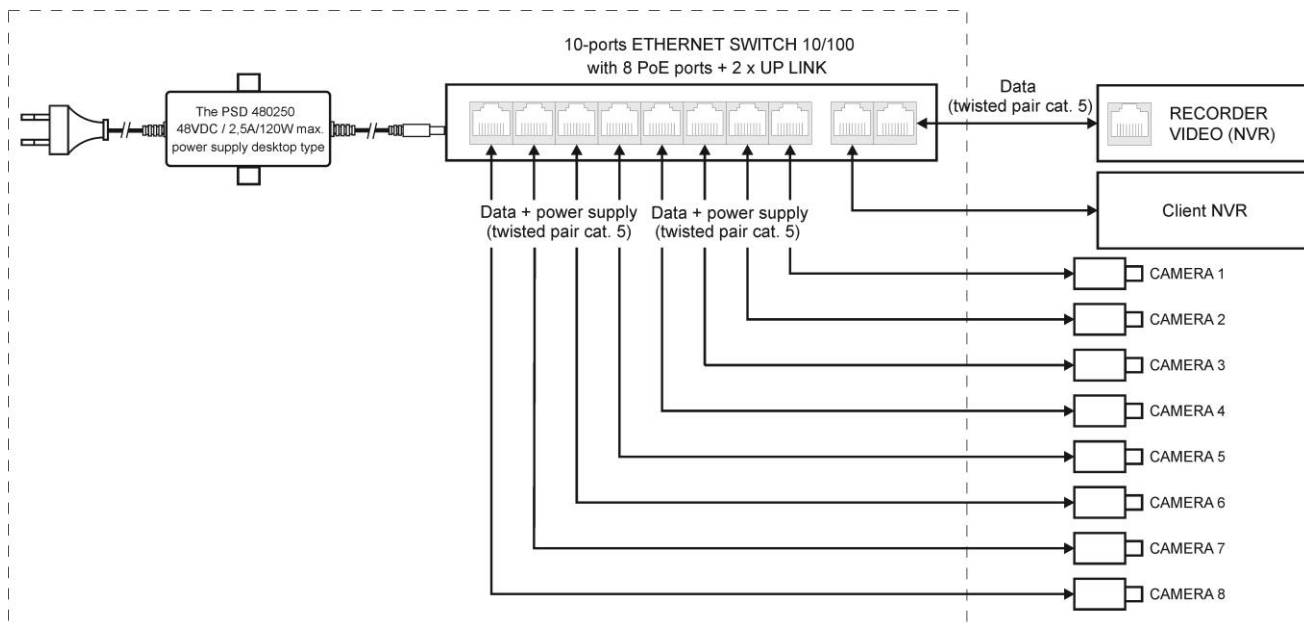
Fig. 1. Block diagram.
