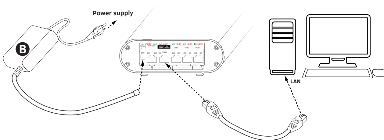
Scheme 1- Power and connect CDS-6IPMulti unit to the computer
